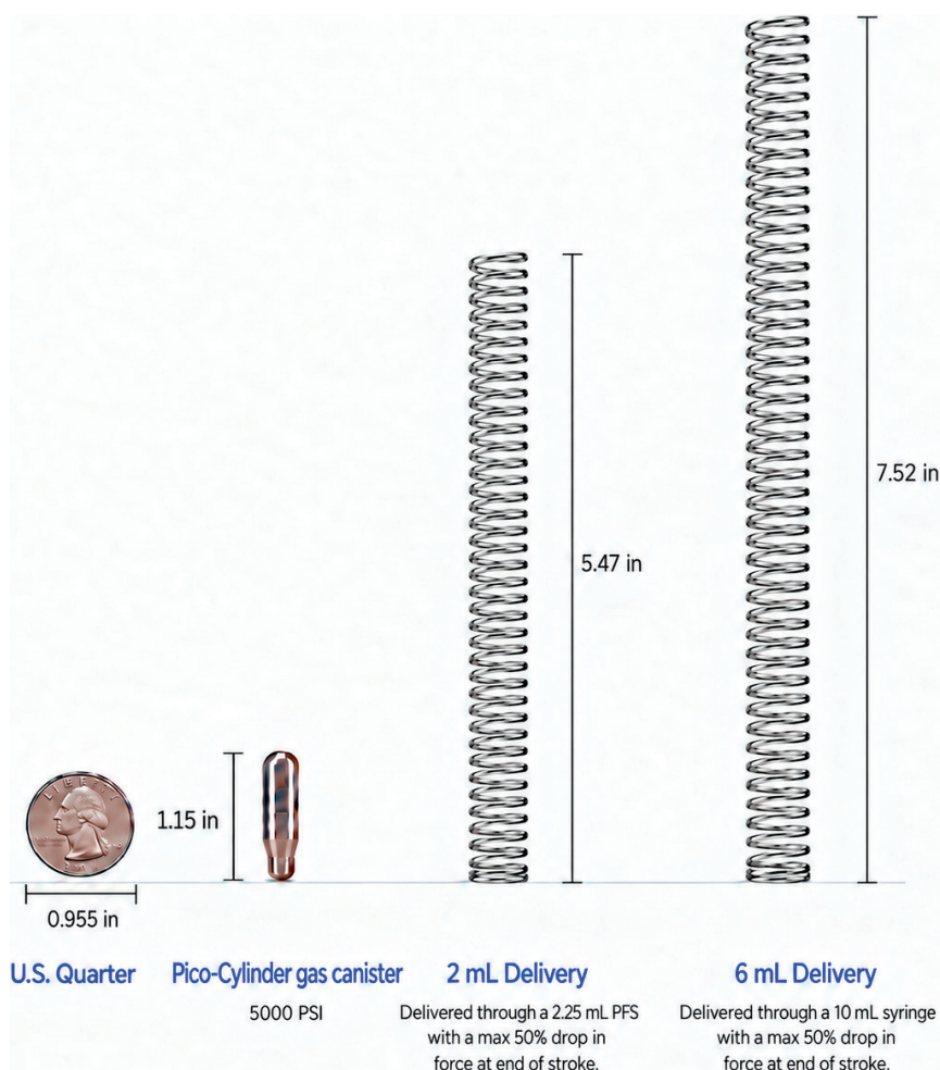
Figure 3: Energy source comparison: the compact gas Pico-Cylinder used in Windgap Medical's platform alongside a mechanical spring of equivalent stored energy. Representative scaling for illustrative purposes.
