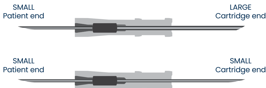
Figure 2: Image inset visualising SHL Medical's split-cannula approach.
