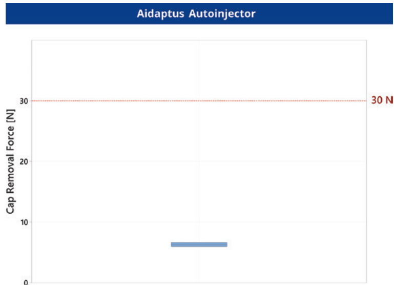
Figure 6: Graph representing cap removal force for Aidaptus autoinjector. No additional effort was required to remove the cap from the syringe, illustrated by the highly consistent results.
