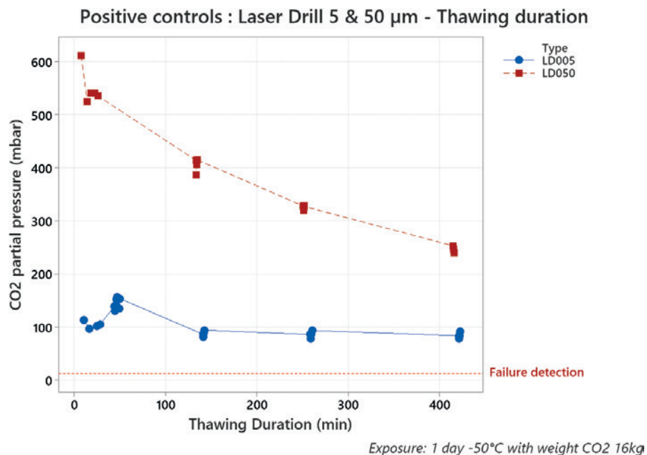
Figure 5: Partial pressure measured in the positive controls samples for different thawing times.
