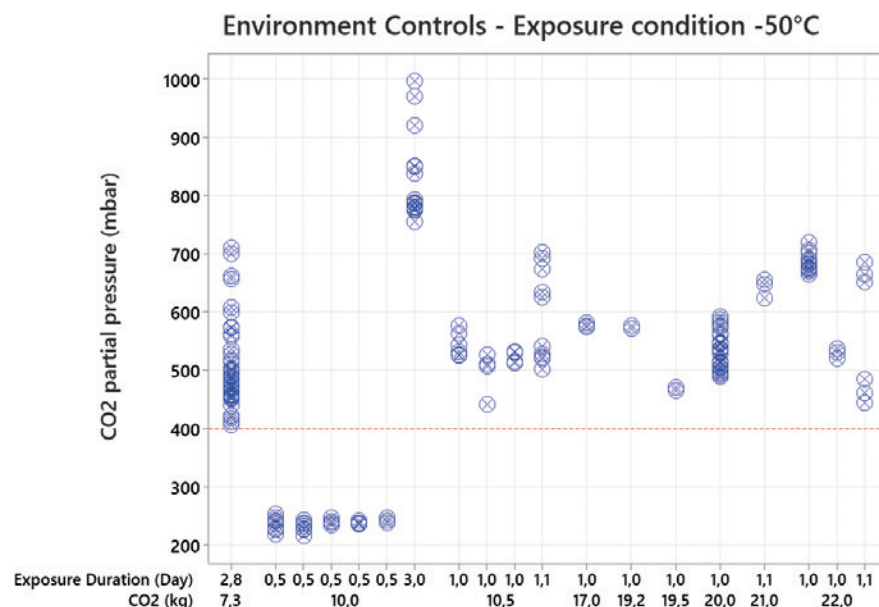
Figure 3: Partial pressure measured in the environmental control samples with different CO 2 gas quantities and exposure times.
