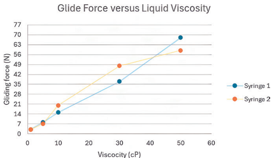
Figure 4: Illustrative glide force response across representative liquid viscosities. Syringe 1 demonstrates a predictable response to increasing viscosity, whereas Syringe 2 shows greater variability. Such trends can provide early insight into system sensitivity and help guide subsequent development activities. Data shown for illustration only.
